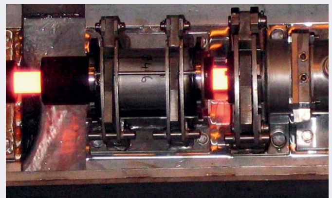
thermocoil® cooling pipe with stripper nozzle.
